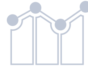
Analytics
